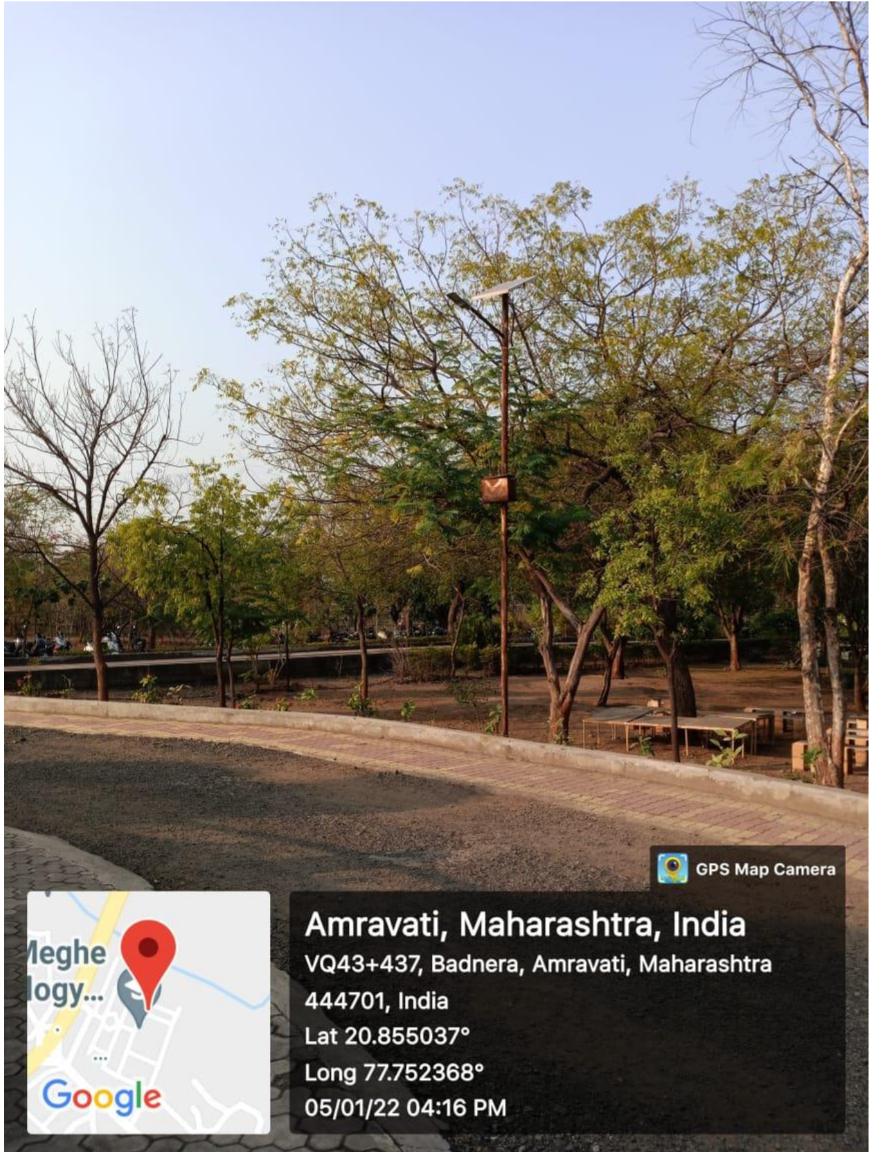
Solar System
